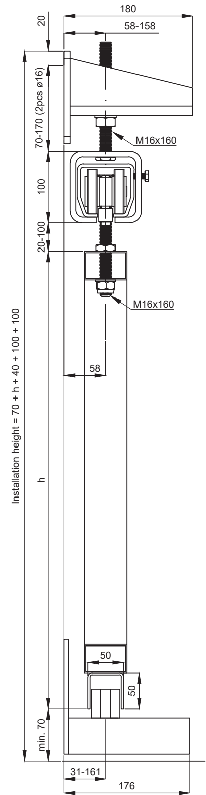
Series 2000 wall fixing
