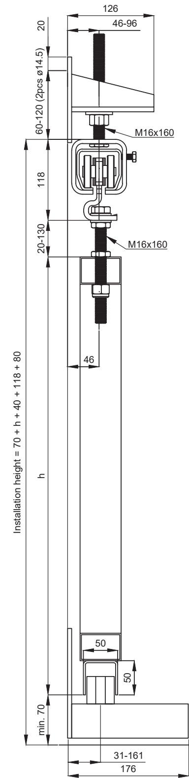
Series 900 wall fixing
