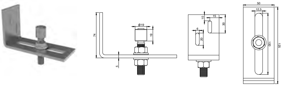
AOK-12, AISI 316 L ø 19 mm. Wall fixing.
