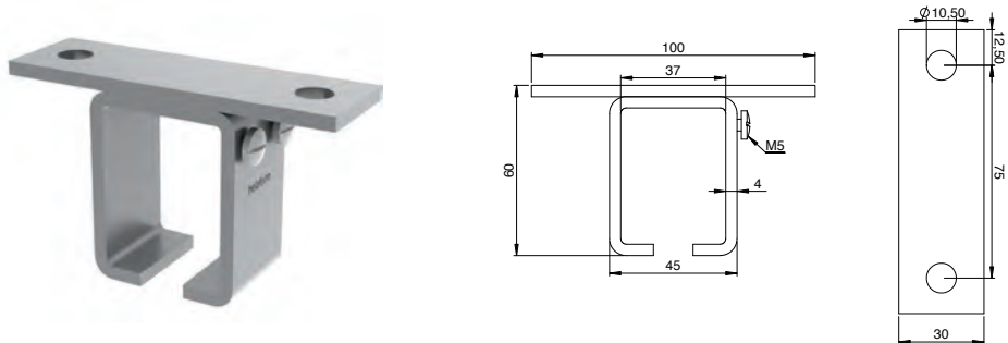
KKK-150 For track K-150. Note! Without joint screws.
