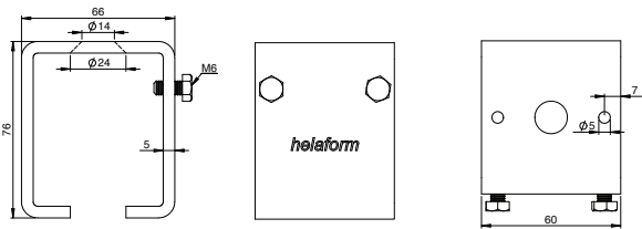
KKL-300/500, AISI 316 L Joint bracket. For tracks K-300 and K-500.
